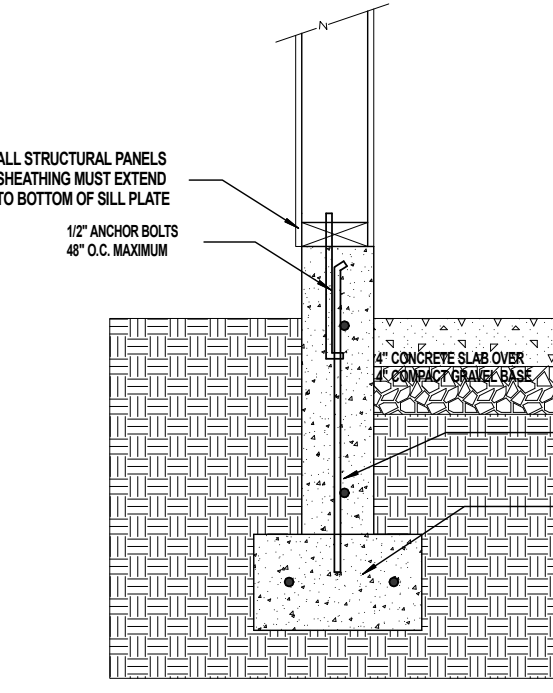
1 GARAGE FOUNDATION DETAIL SCALE: 3/4"=1'0"
